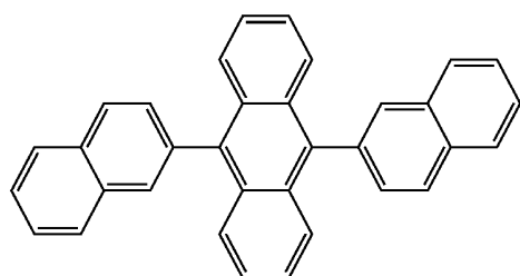
Compound 1
