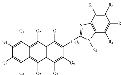
Formula 3
