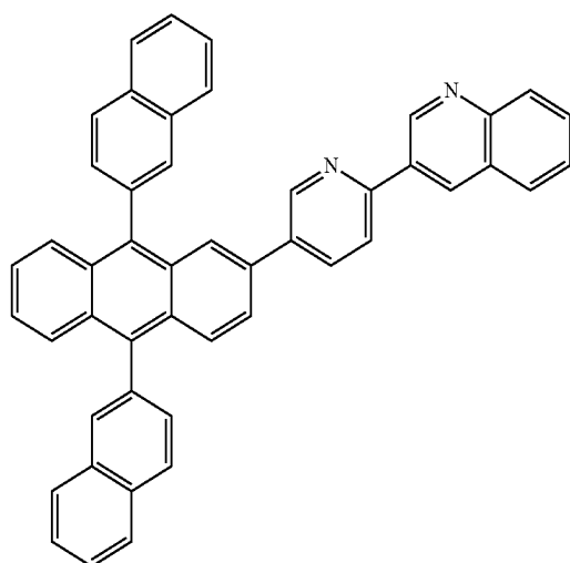
Compound 7
