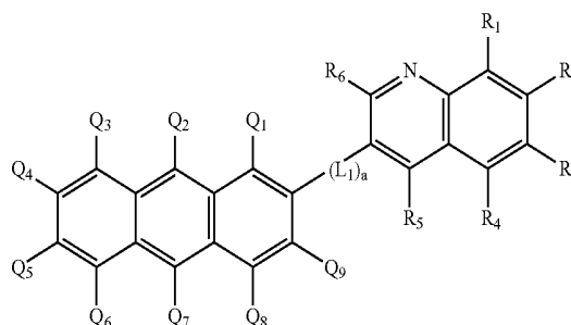
Formula 3
