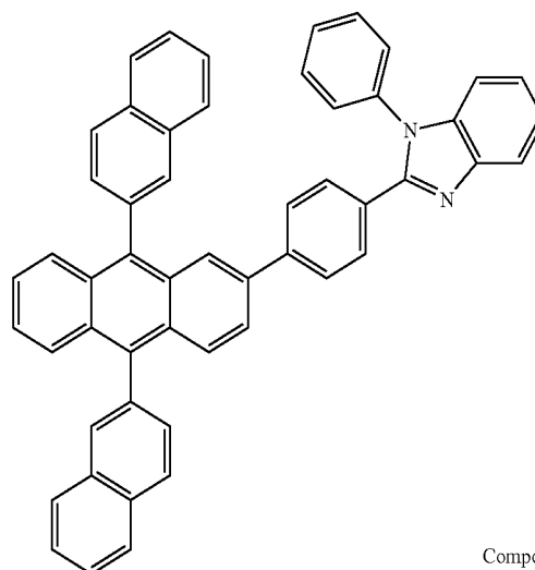
Compound 6
